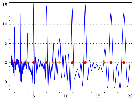
S_\rho(x) summed over 50 zeta zeros.
