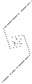
Quadratic form (x^2 + x + 41) primes and not primes.
